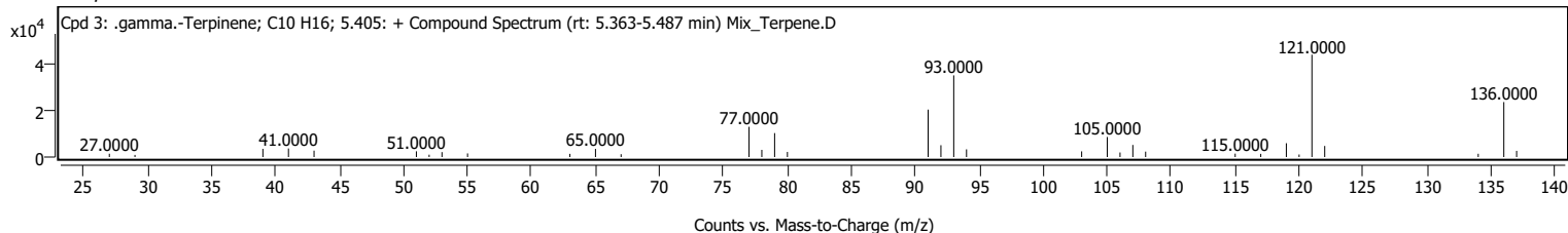
Observed Spectrum
