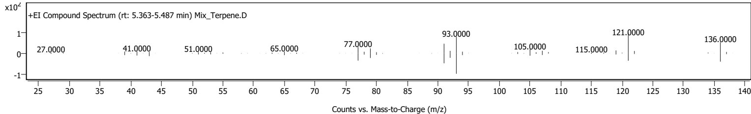
Library Spectrum
