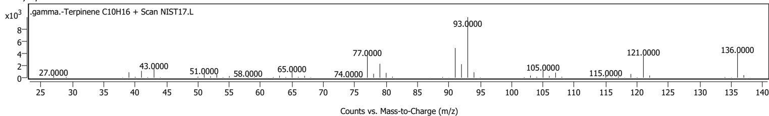
Library Spectrum
